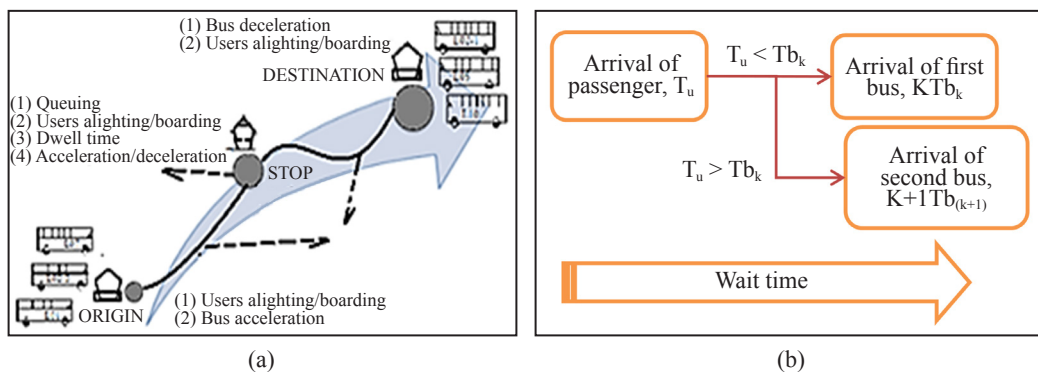
Figure 2. (a) Location of bus delays; and (b) flowchart of passenger arrival time at random Note: T_u , arrival time of passenger; T b_k , arrival time of first bus; and T b_{(k+1)} , arrival time of second bus
